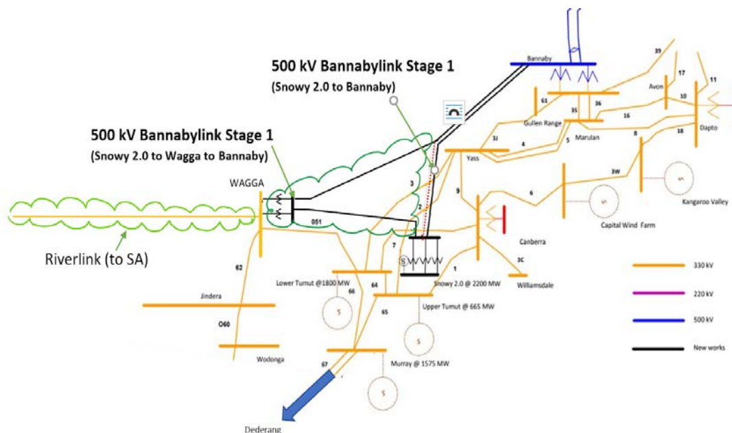
Figure 12: TransGrid Option 10 (new 500 kV lines and switchyard) (Feasibility Study 2017)
