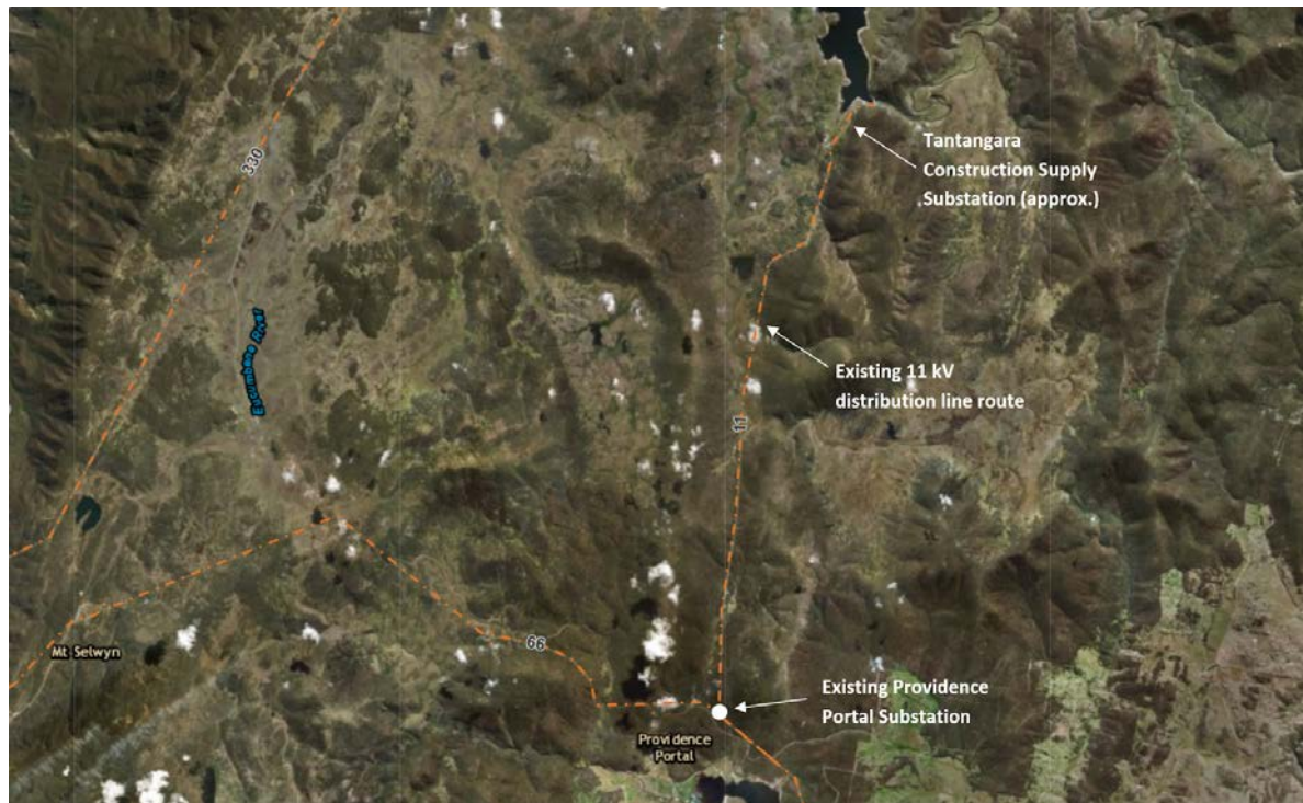
Figure 24: Tantangara construction supply
