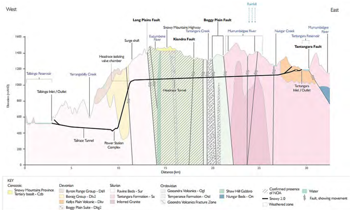
Figure 2-2 Natural Rock Domains Showing Confirmed Presence of NOA
