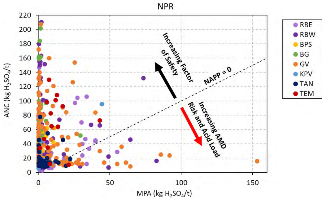
Figure 4-1 ABA plot for the samples collected to mid-January 2022
