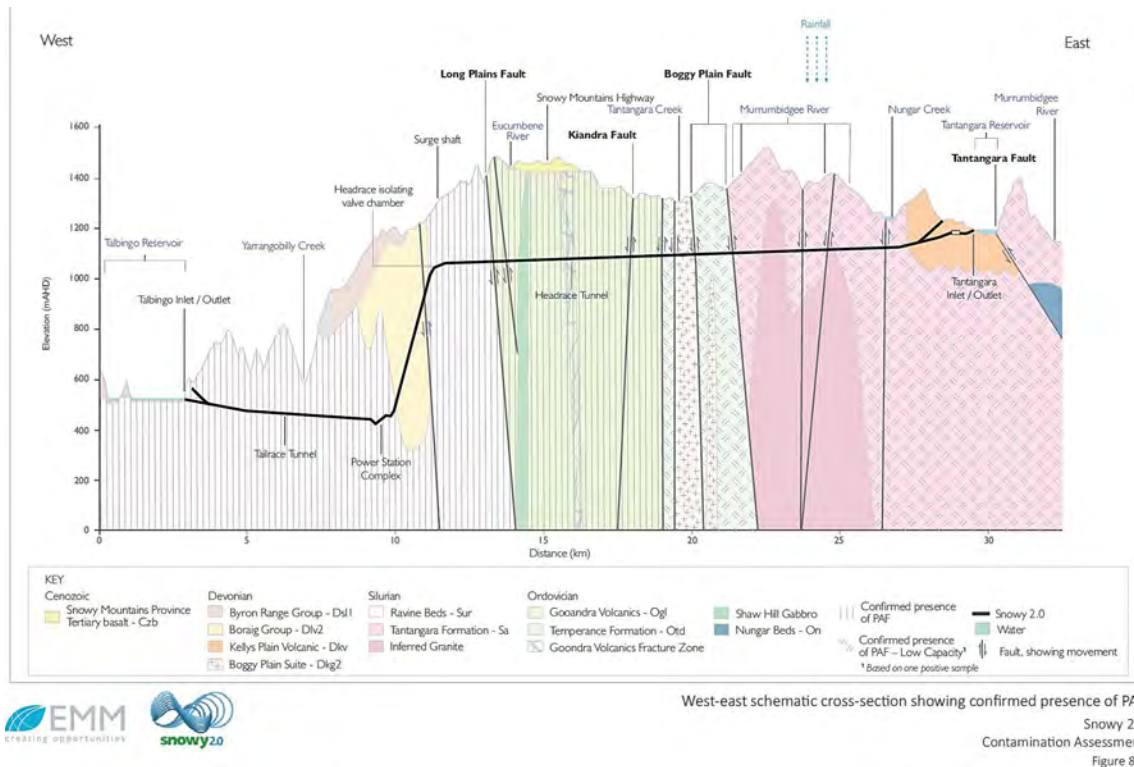
Figure 1-1 West-East cross section showing confirmed presence of PAF material
