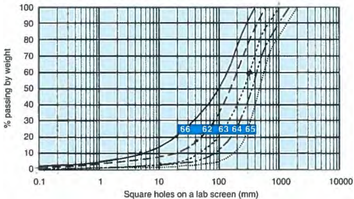
Figure 4-8: Raw material curves for drill and blast (Bellopede R et al 2011)
