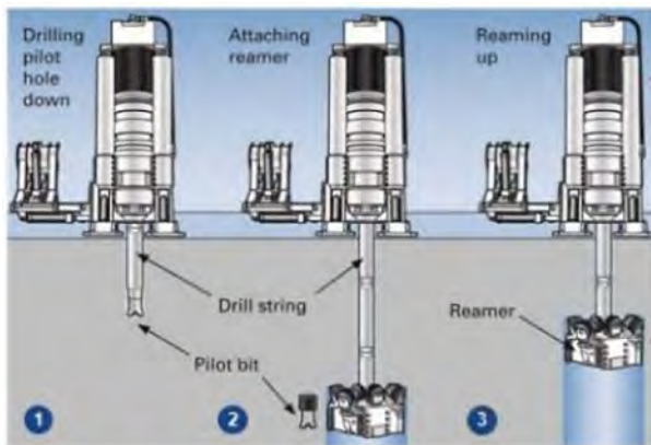
Raise boring
