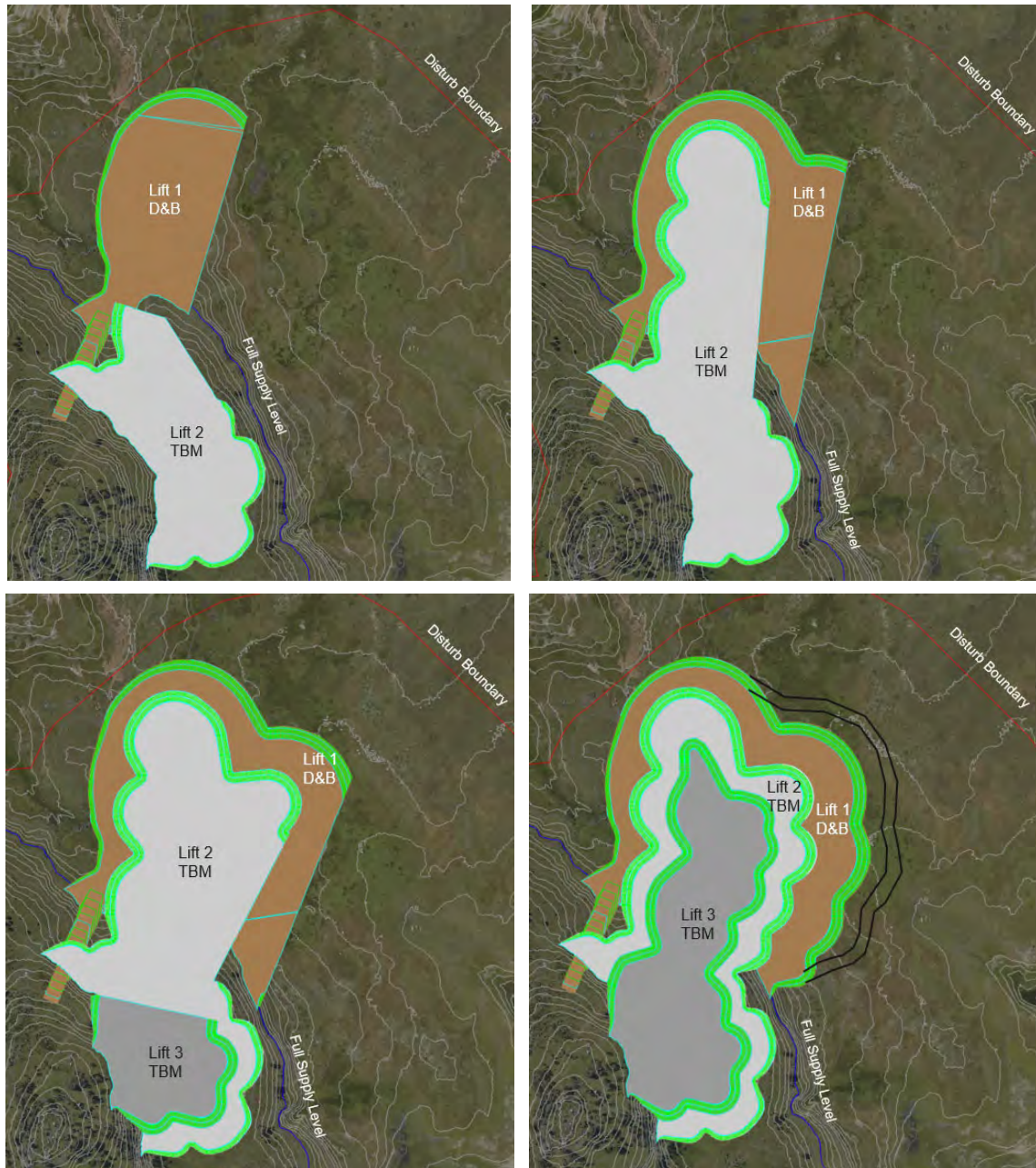
Figure 4-2 Indicative construction sequence, Tantangara PSE
