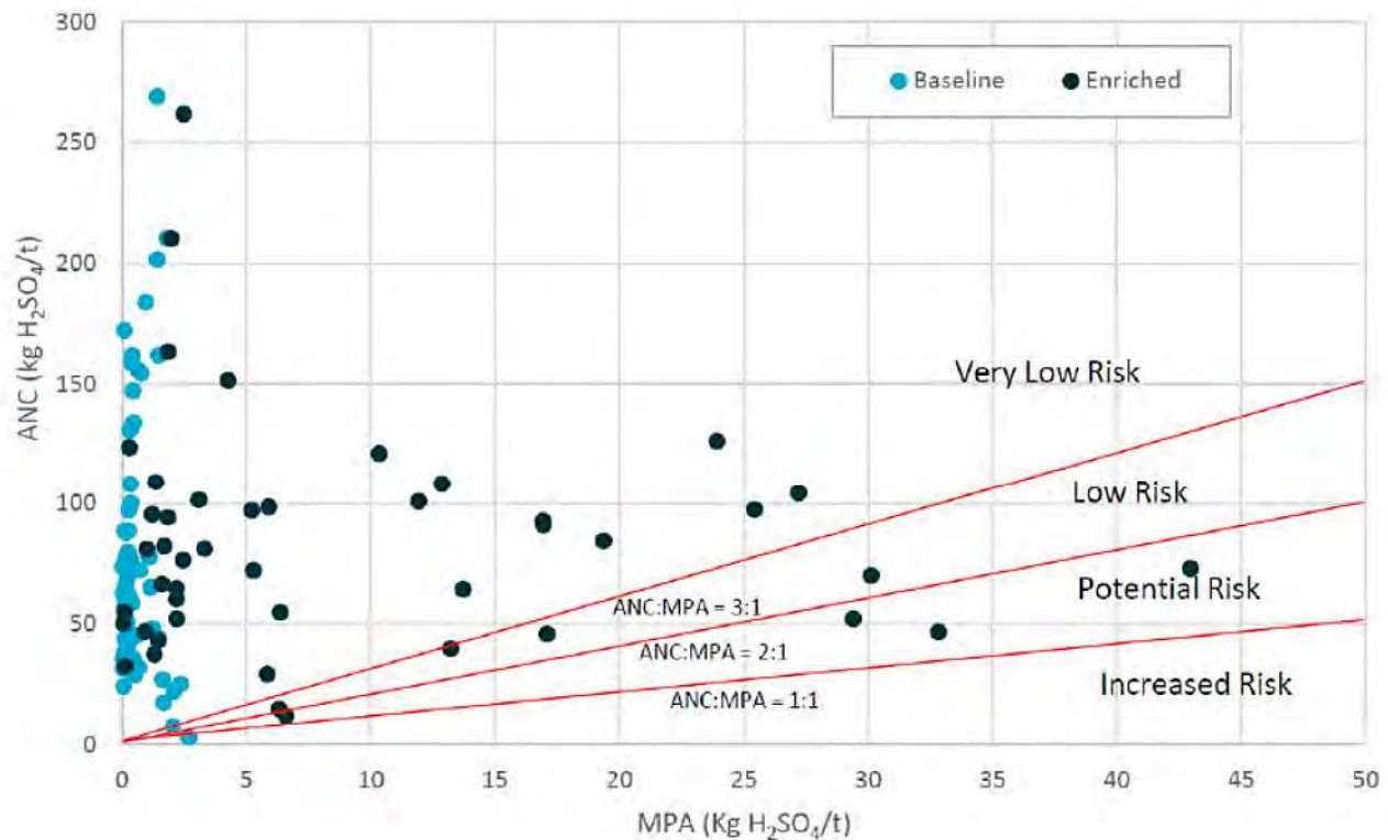
Figure 3-3: Categorisation of ANC versus MPA risk (source: EIS Appendix L, Annexure B)
