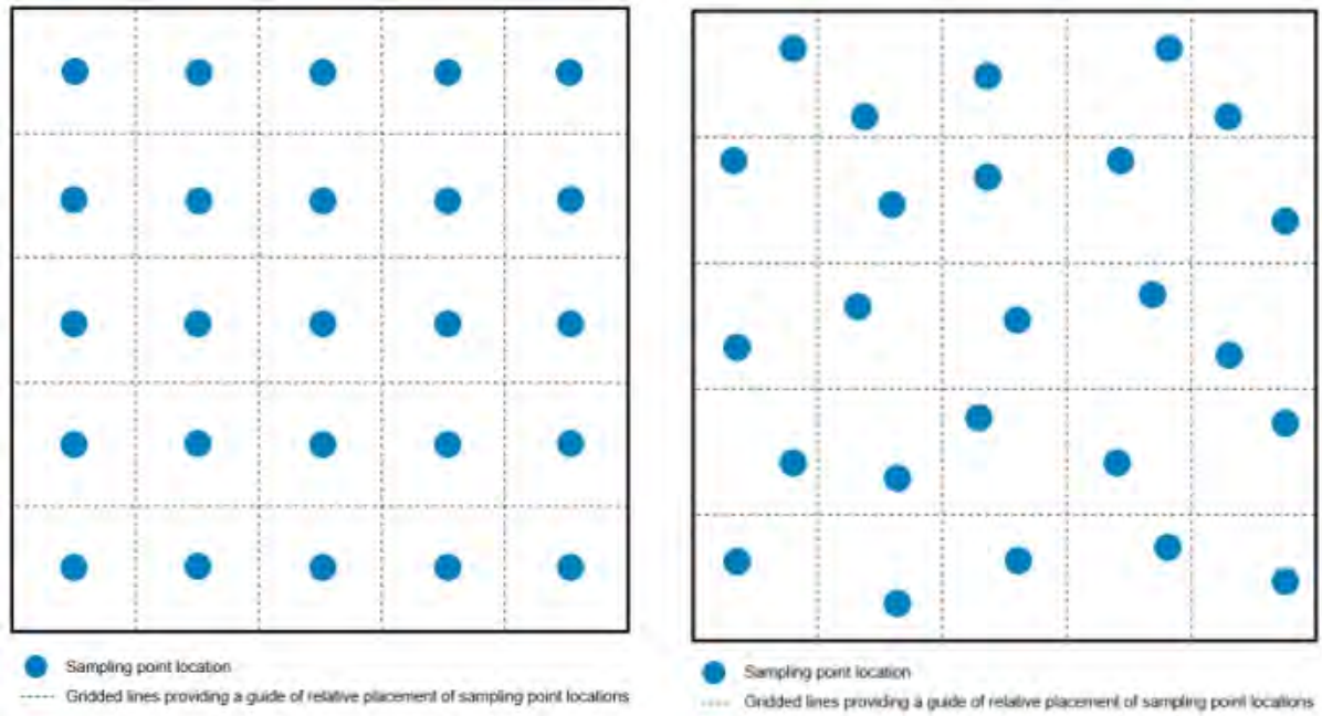
Figure 3-1 Example of Emplacement Area Sampling
