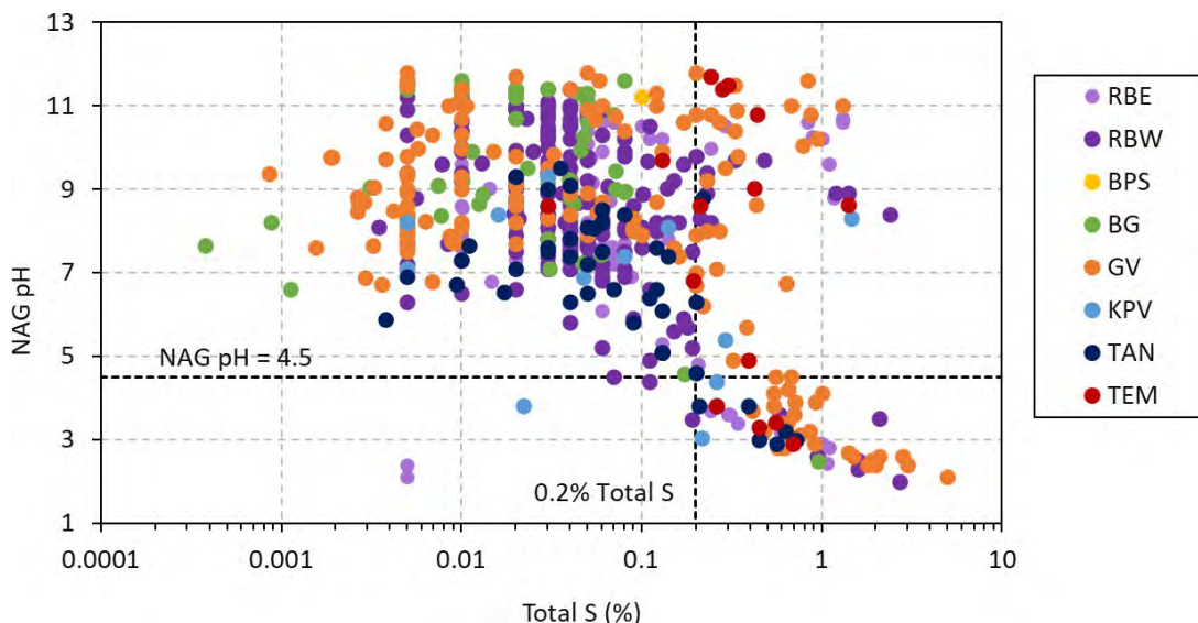
Figure 5-1 Site sulfur cut-off based on NAG pH 4.5
