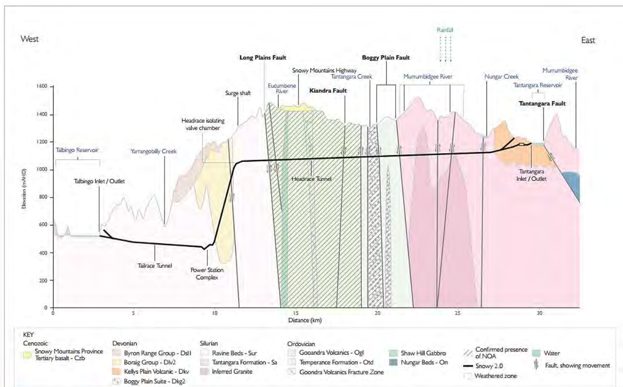
West-east schematic cross-section showing confirmed presence of NOA
