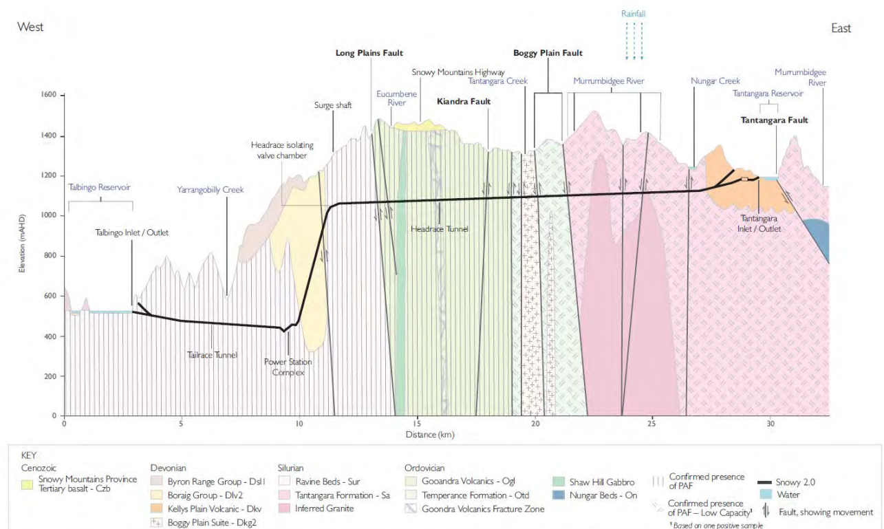
Figure 2-1 Natural Rock Domains Showing Confirmed Presence of PAF
