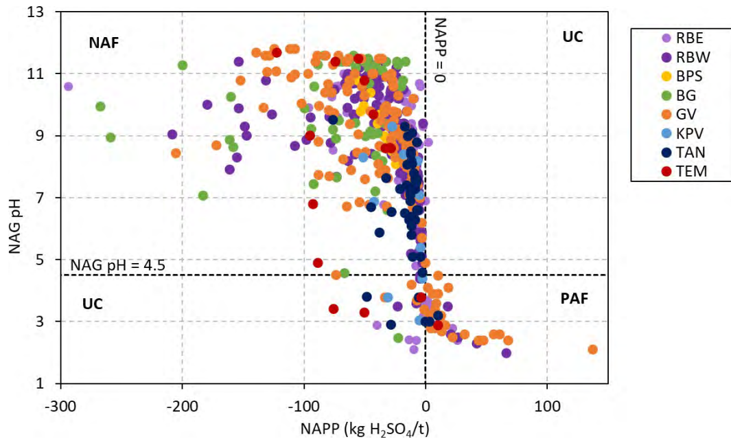
Figure 4-2 Classification for each geological unit using AMIRA International, 2002
