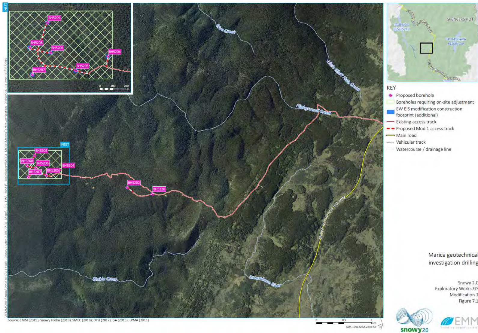
Figure 4 | Location of Approved Exploratory Works - Boreholes
