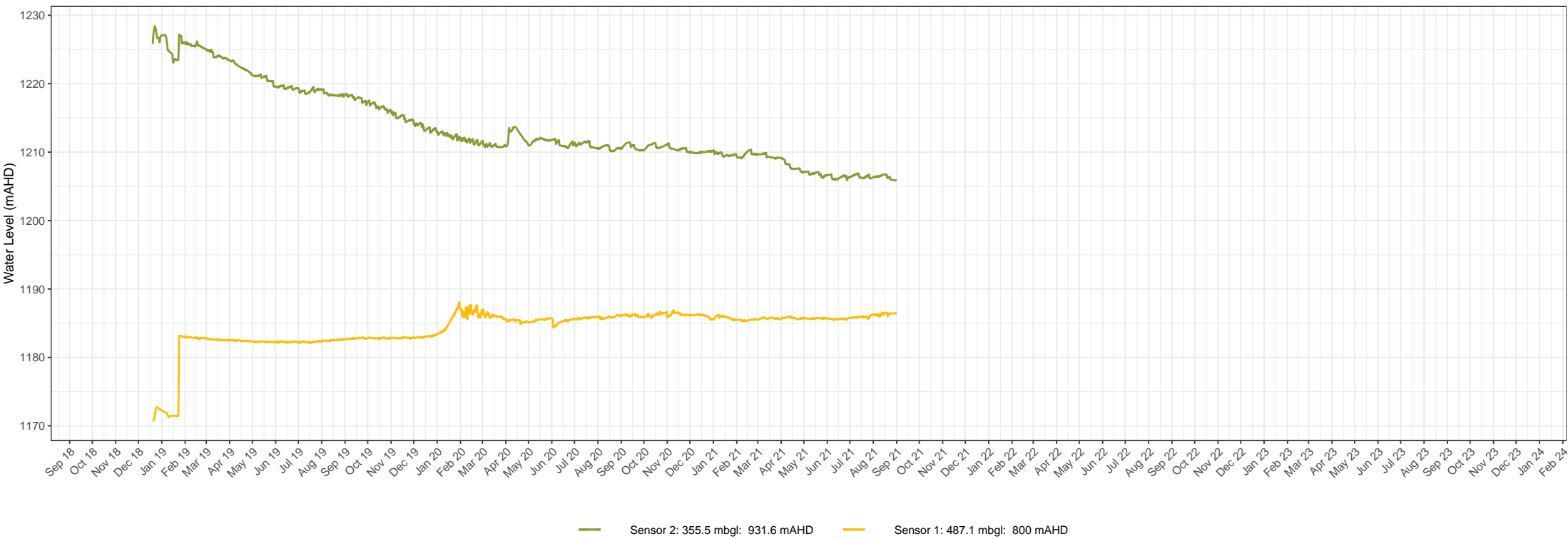
BH5114 groundwater level times series data Snowy Hydro 2.0 – Snowy Hydro Limited Groundwater monitoring and management Figure 1. 24
