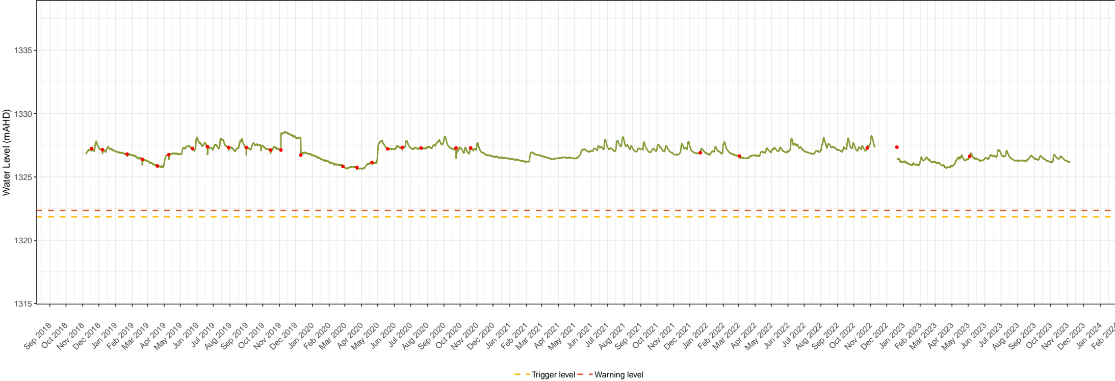
MB04B groundwater level times series data Snowy 2.0 – Snowy Hydro Limited Groundwater monitoring and management Figure 1. 30
