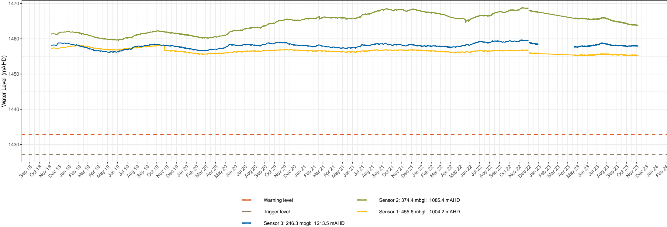
BH4102 groundwater level times series data Snowy Hydro 2.0 – Snowy Hydro Limited Groundwater monitoring and management Figure 1. 10
