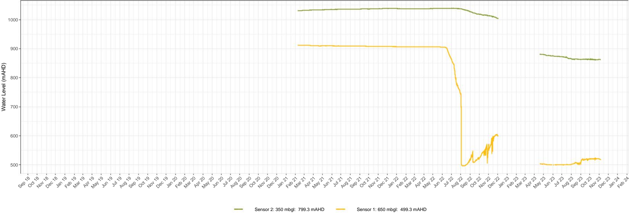
BH5209 groundwater level times series data Snowy Hydro 2.0 – Snowy Hydro Limited Groundwater monitoring and management Figure 1. 32
