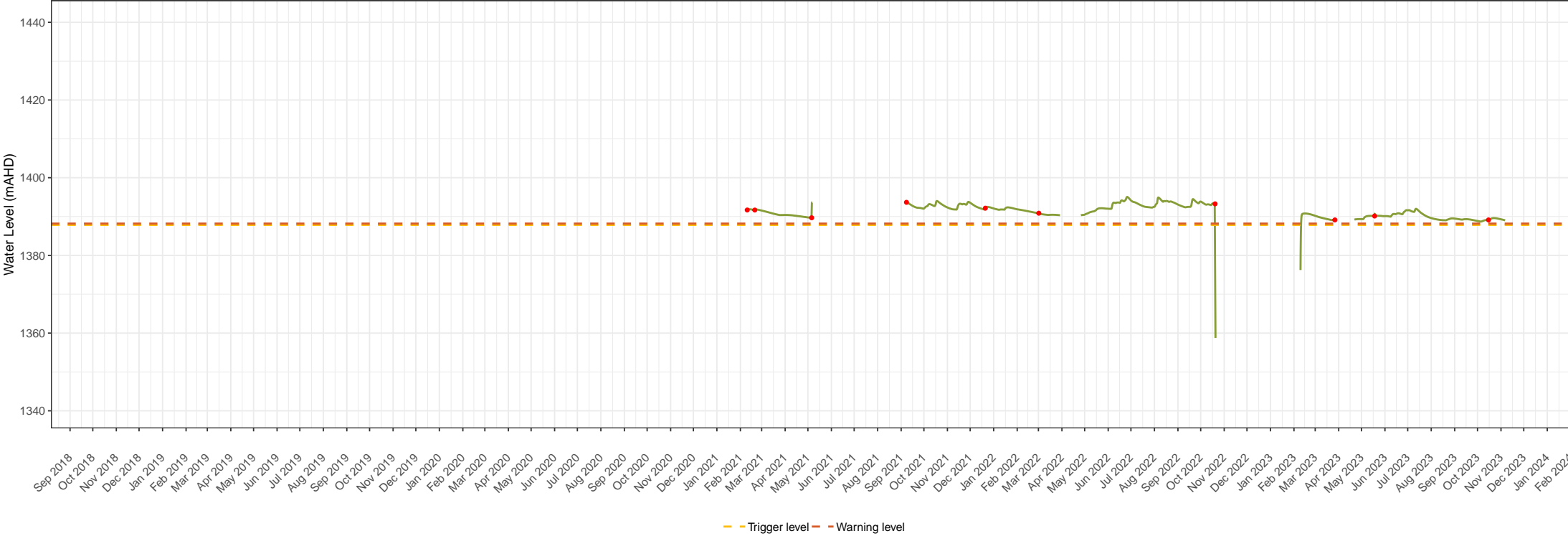
RtS_BH2B groundwater level times series data Snowy 2.0 – Snowy Hydro Limited Groundwater monitoring and management Figure 1. 71
