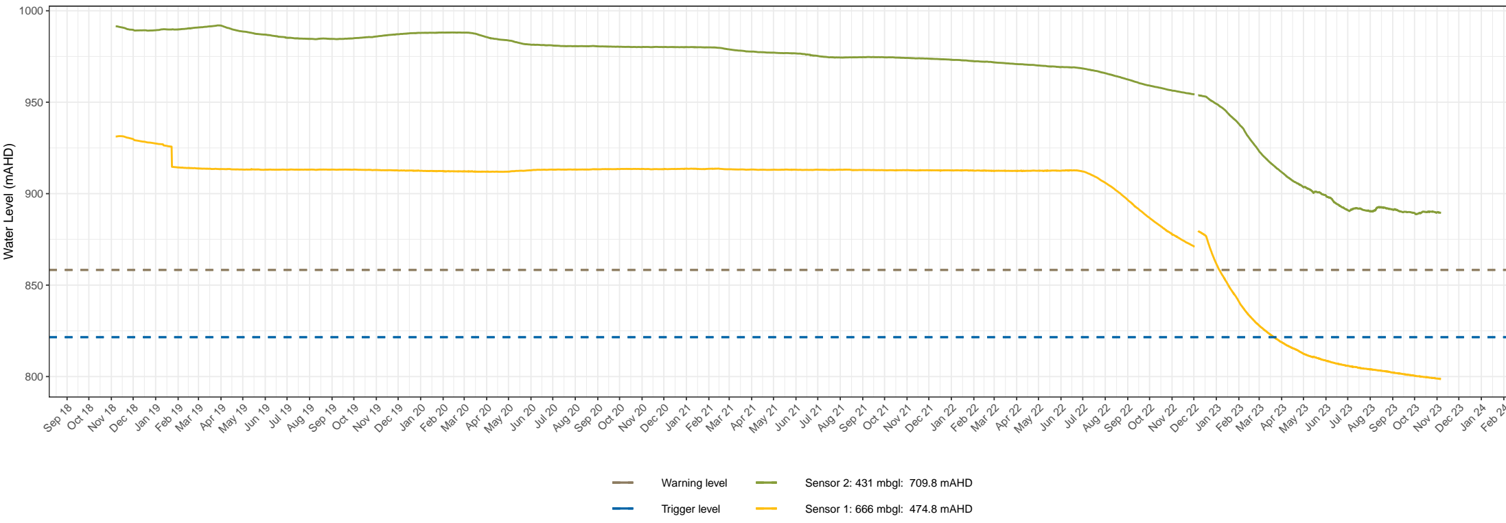
BH5108 groundwater level times series data Snowy Hydro 2.0 – Snowy Hydro Limited Groundwater monitoring and management Figure 1. 19
