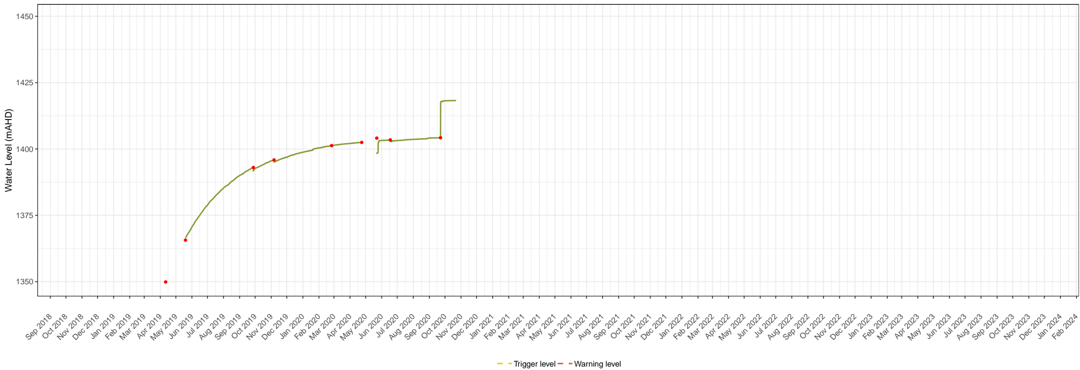
PB06 groundwater level times series data Snowy 2.0 – Snowy Hydro Limited Groundwater monitoring and management Figure 1. 49
