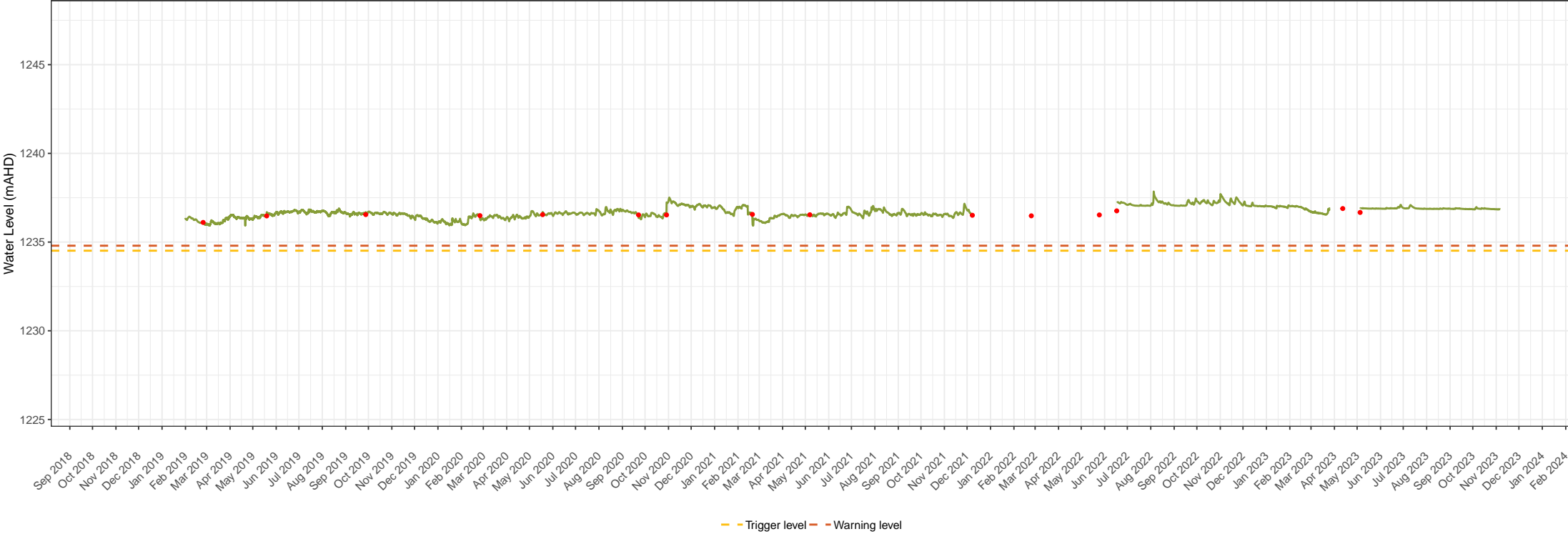
NC03 groundwater level times series data Snowy 2.0 – Snowy Hydro Limited Groundwater monitoring and management Figure 1. 44
