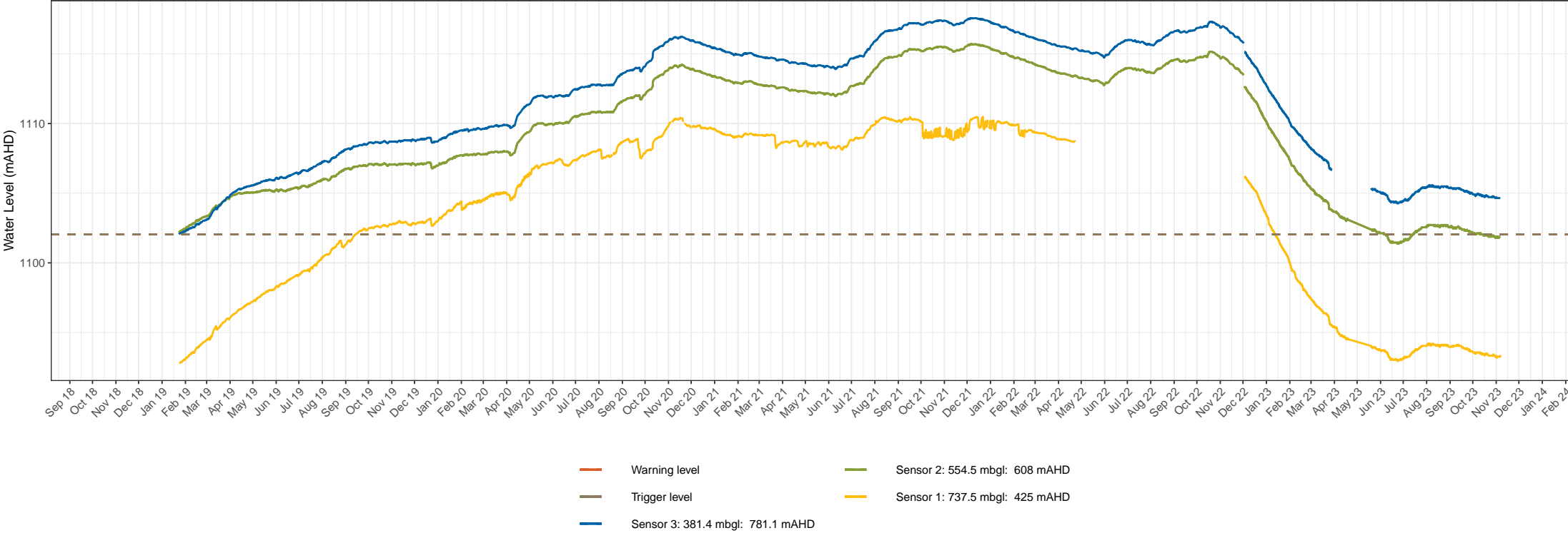
BH5107 groundwater level times series data Snowy Hydro 2.0 – Snowy Hydro Limited Groundwater monitoring and management Figure 1. 18
