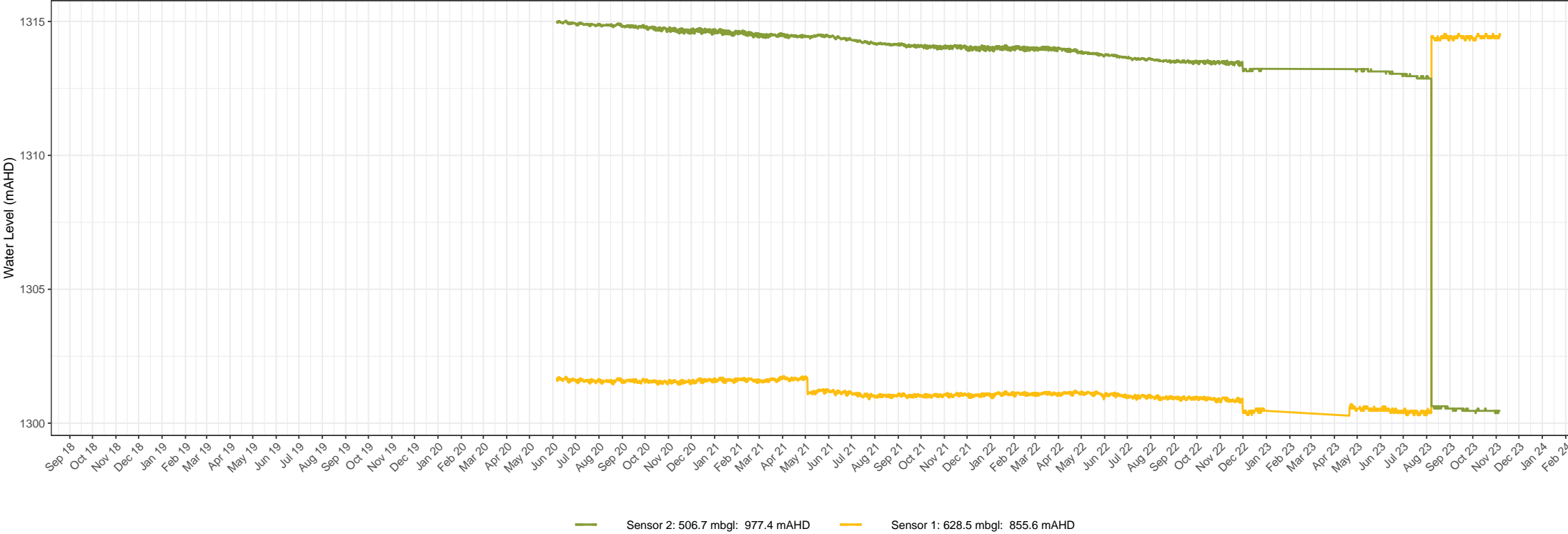
BH4104 groundwater level times series data Snowy Hydro 2.0 – Snowy Hydro Limited Groundwater monitoring and management Figure 1. 12
