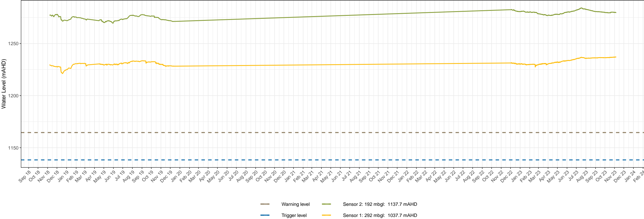
BH5115 groundwater level times series data Snowy Hydro 2.0 – Snowy Hydro Limited Groundwater monitoring and management Figure 1. 25
