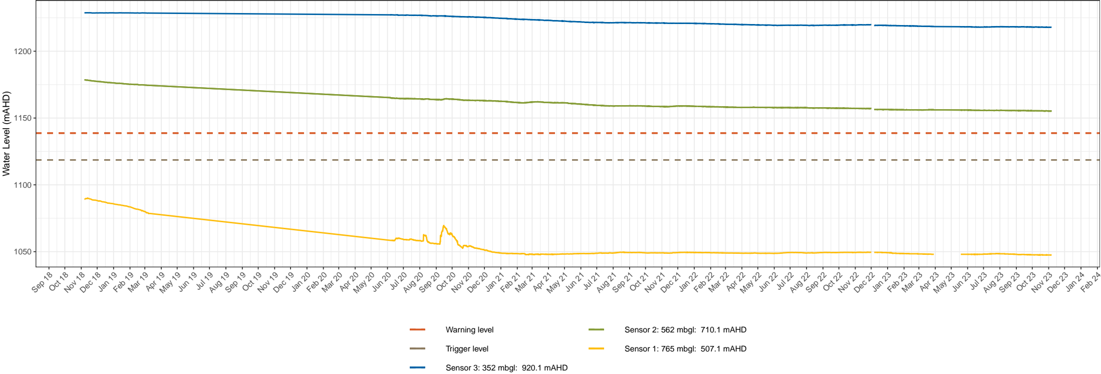
BH5103 groundwater level times series data Snowy Hydro 2.0 – Snowy Hydro Limited Groundwater monitoring and management Figure 1. 16
