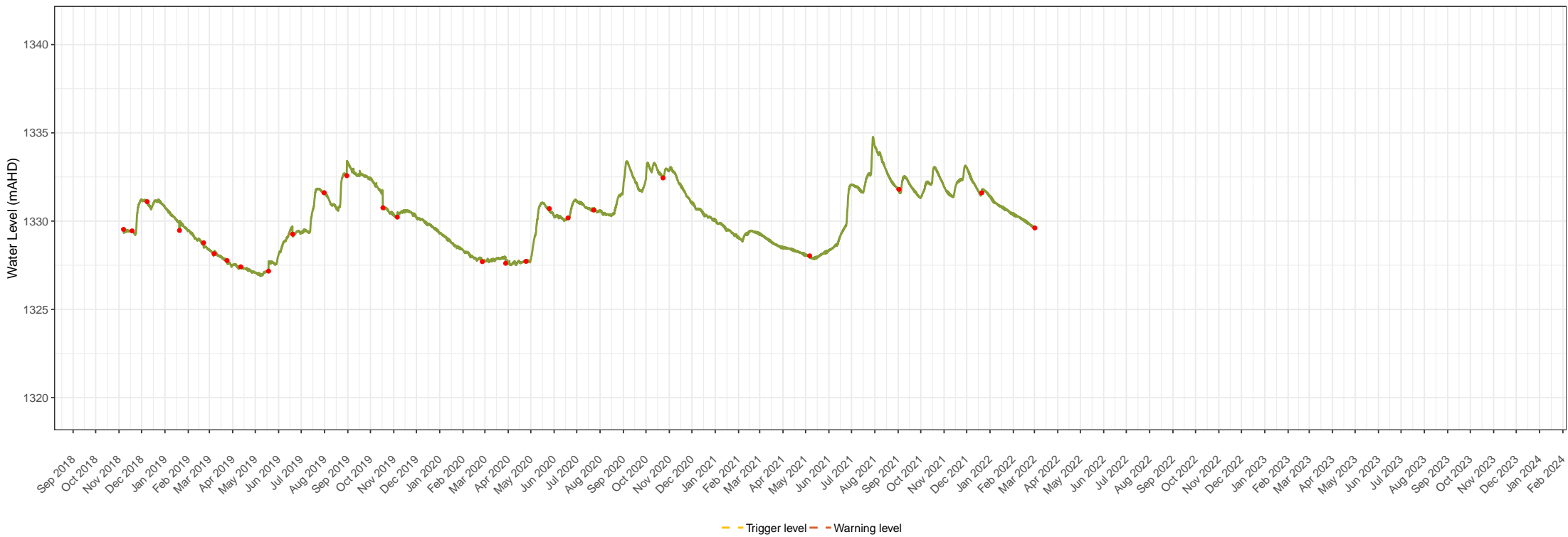
TMB04 groundwater level times series data Snowy 2.0 – Snowy Hydro Limited Groundwater monitoring and management Figure 1. 97
