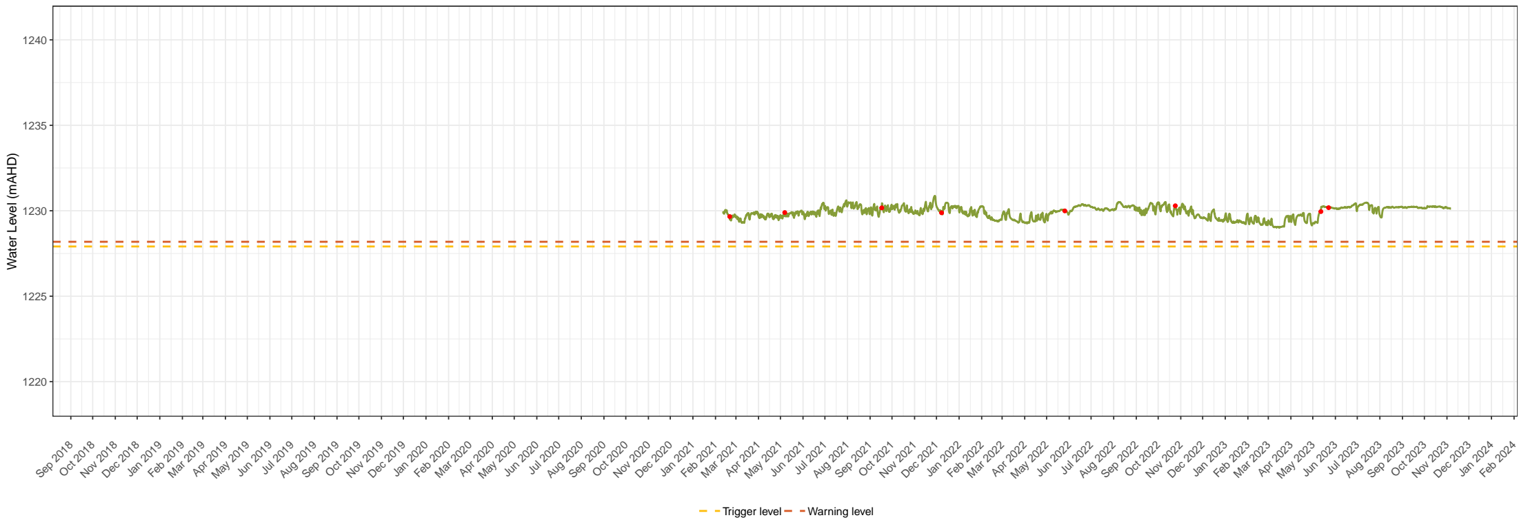
RtS_BH7B groundwater level times series data Snowy 2.0 – Snowy Hydro Limited Groundwater monitoring and management Figure 1. 79
