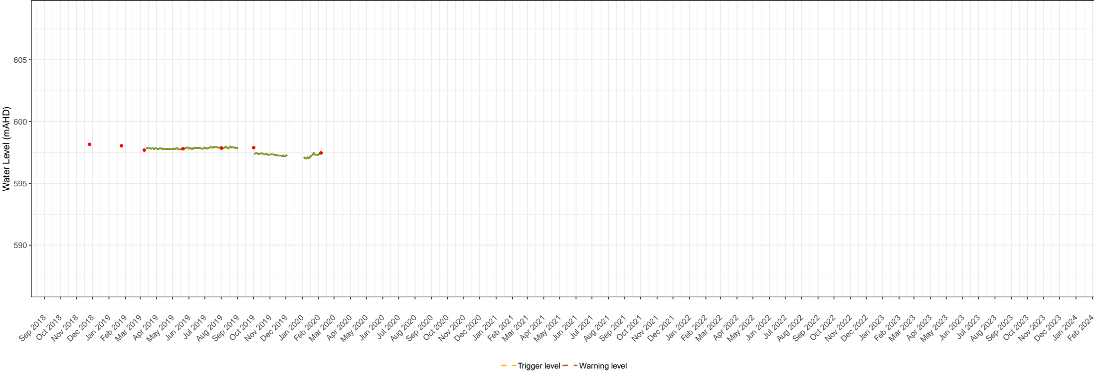
BH8105 groundwater level times series data Snowy 2.0 – Snowy Hydro Limited Groundwater monitoring and management Figure 1. 19
