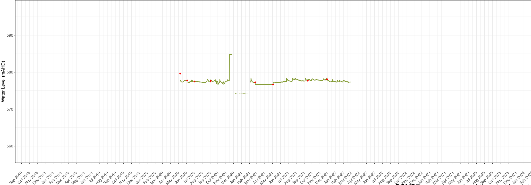
R SMB7 groundwater level times series data Snowy 2.0 – Snowy Hydro Limited Groundwater monitoring and management Figure 1. 53
