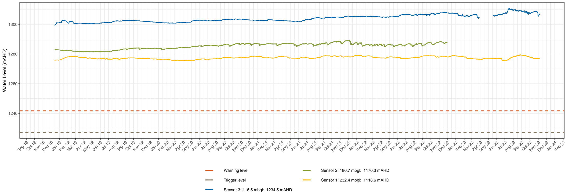
BH5111 groundwater level times series data Snowy Hydro 2.0 – Snowy Hydro Limited Groundwater monitoring and management Figure 1. 21
