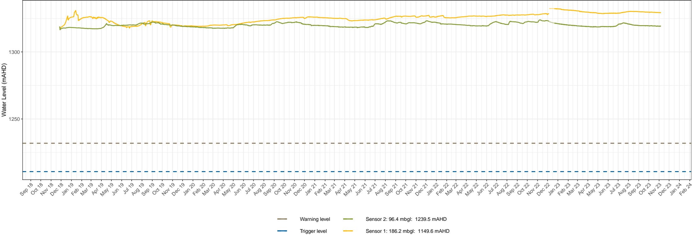
BH3113 groundwater level times series data Snowy Hydro 2.0 – Snowy Hydro Limited Groundwater monitoring and management Figure 1.7
