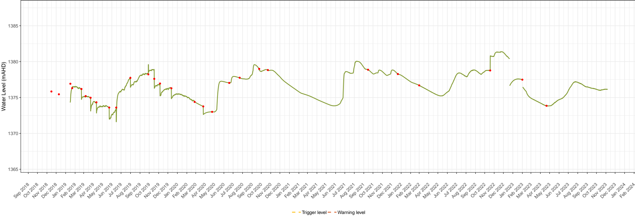
MB13A groundwater level times series data Snowy 2.0 – Snowy Hydro Limited Groundwater monitoring and management Figure 1. 40
