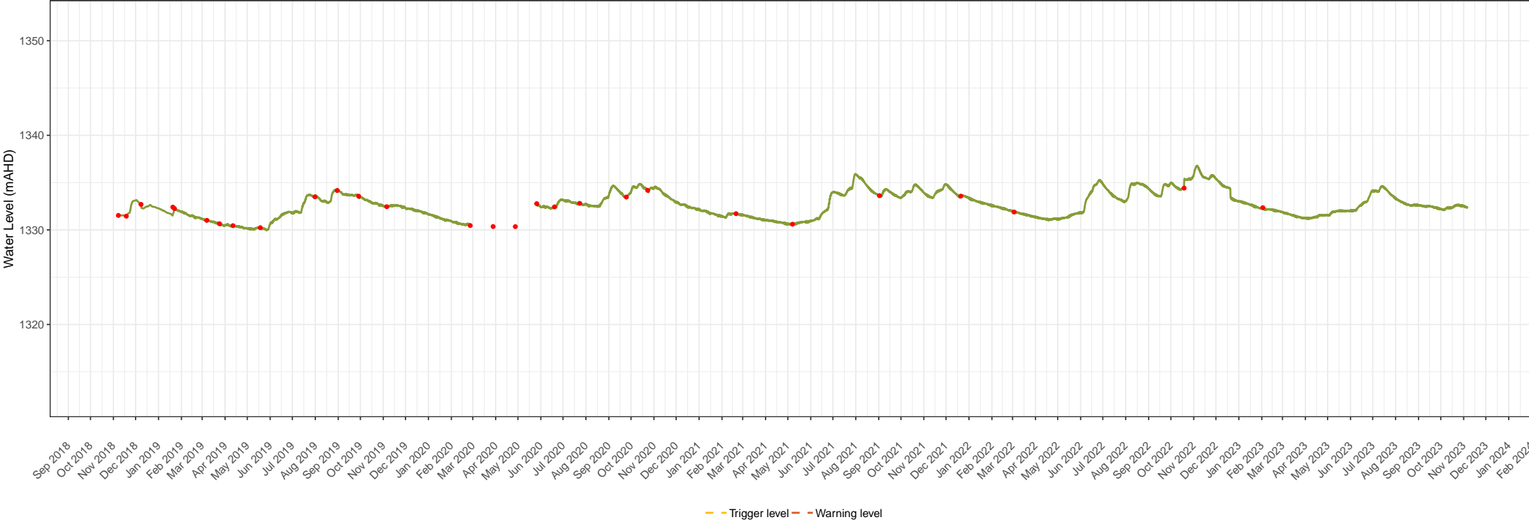
PB04 groundwater level times series data Snowy 2.0 – Snowy Hydro Limited Groundwater monitoring and management Figure 1. 47
