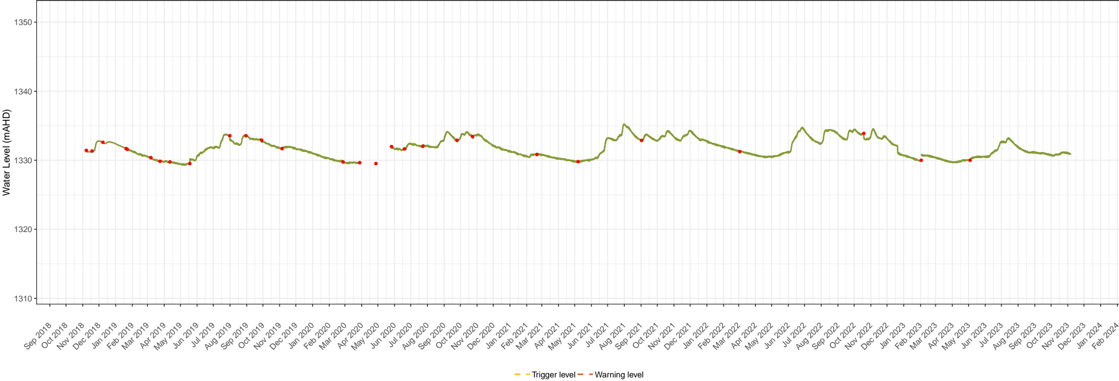
SMB04 groundwater level times series data Snowy 2.0 – Snowy Hydro Limited Groundwater monitoring and management Figure 1. 87
