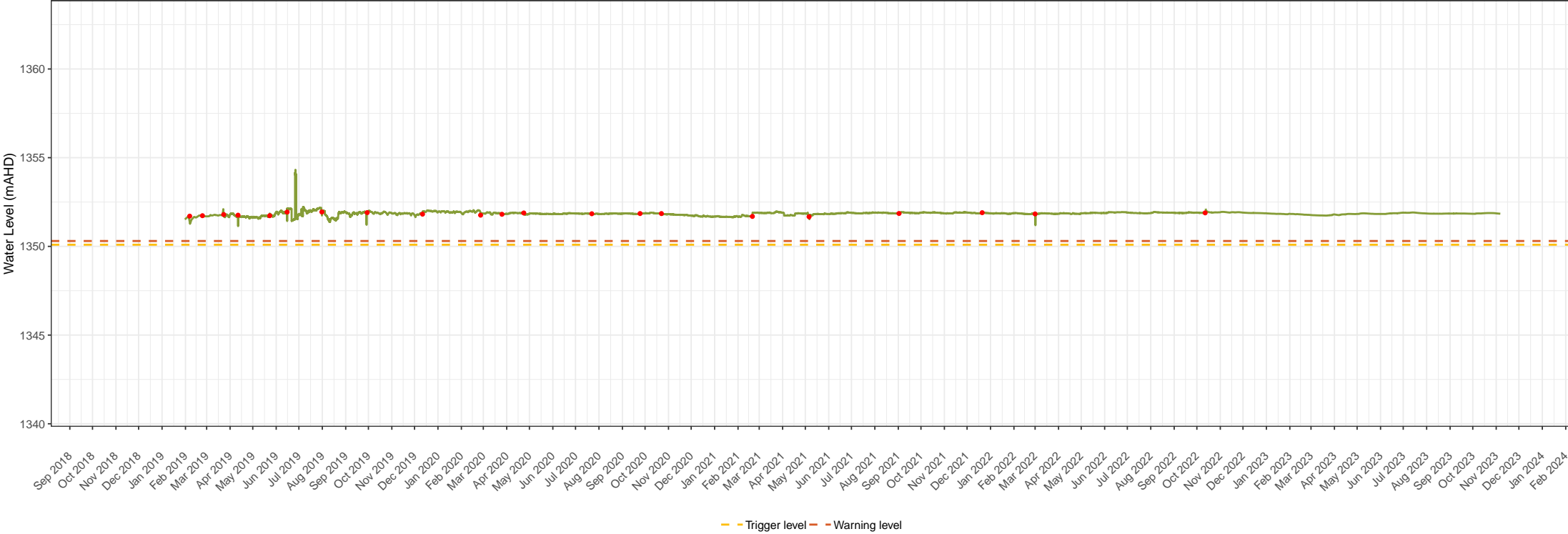
BH02 groundwater level times series data Snowy 2.0 – Snowy Hydro Limited Groundwater monitoring and management Figure 1.2
