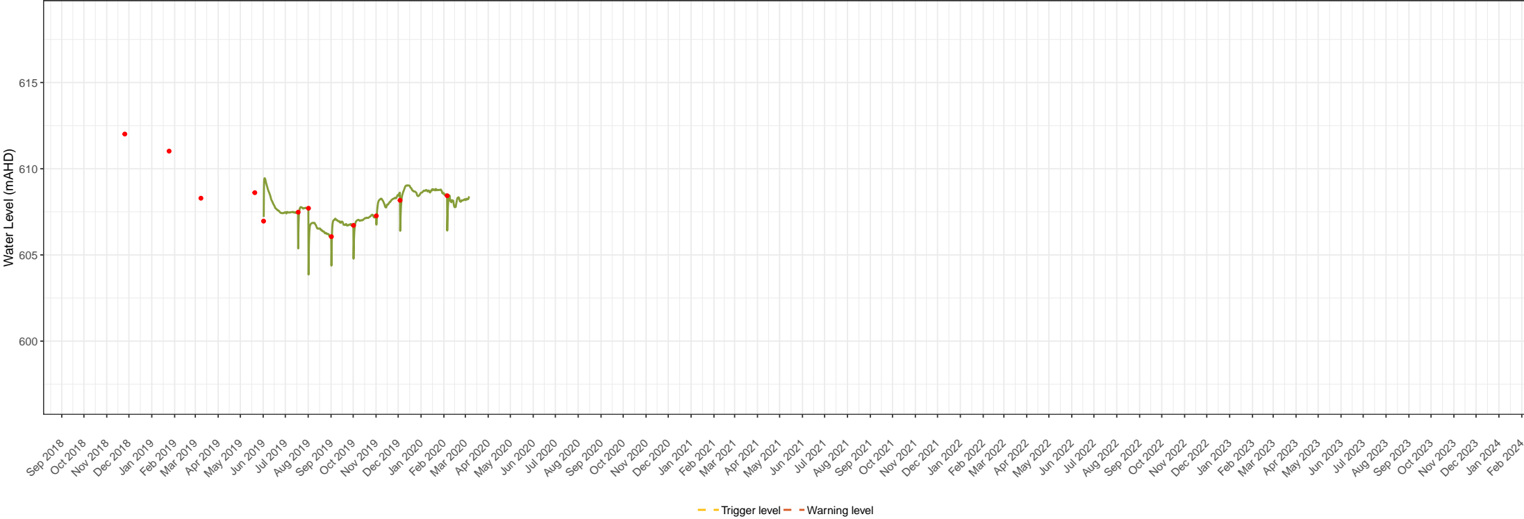
BH8108 groundwater level times series data Snowy 2.0 – Snowy Hydro Limited Groundwater monitoring and management Figure 1. 20
