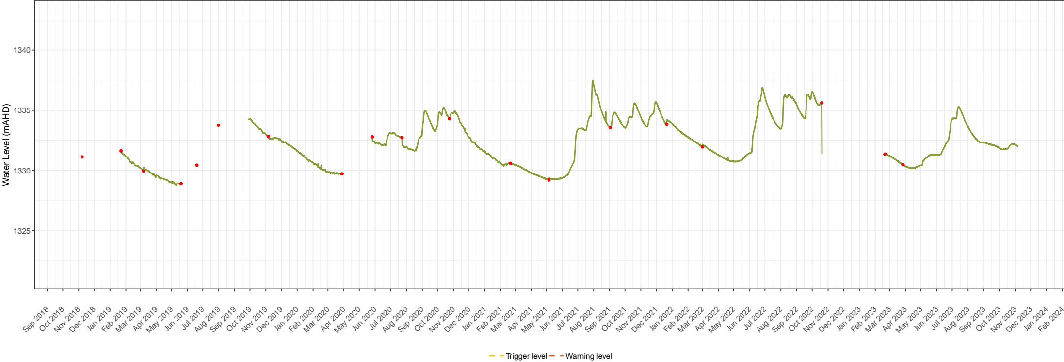
BH3110 groundwater level times series data Snowy 2.0 – Snowy Hydro Limited Groundwater monitoring and management Figure 1. 11
