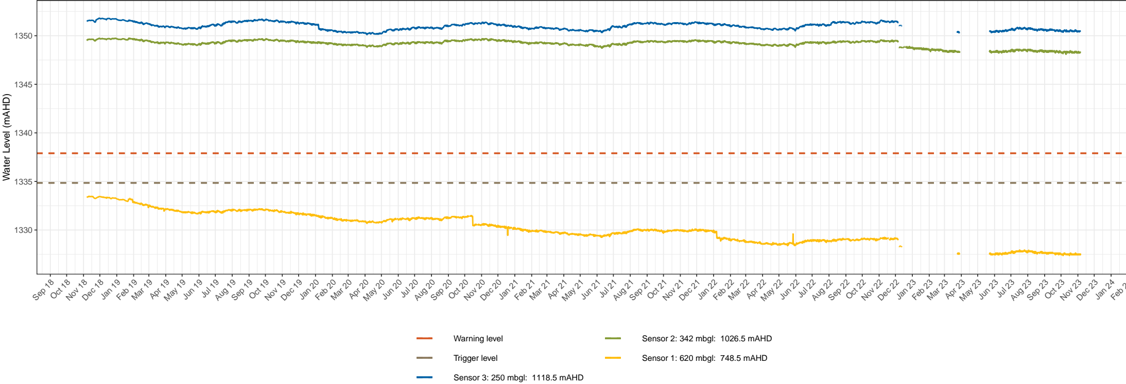
BH3108 groundwater level times series data Snowy Hydro 2.0 – Snowy Hydro Limited Groundwater monitoring and management Figure 1.5
