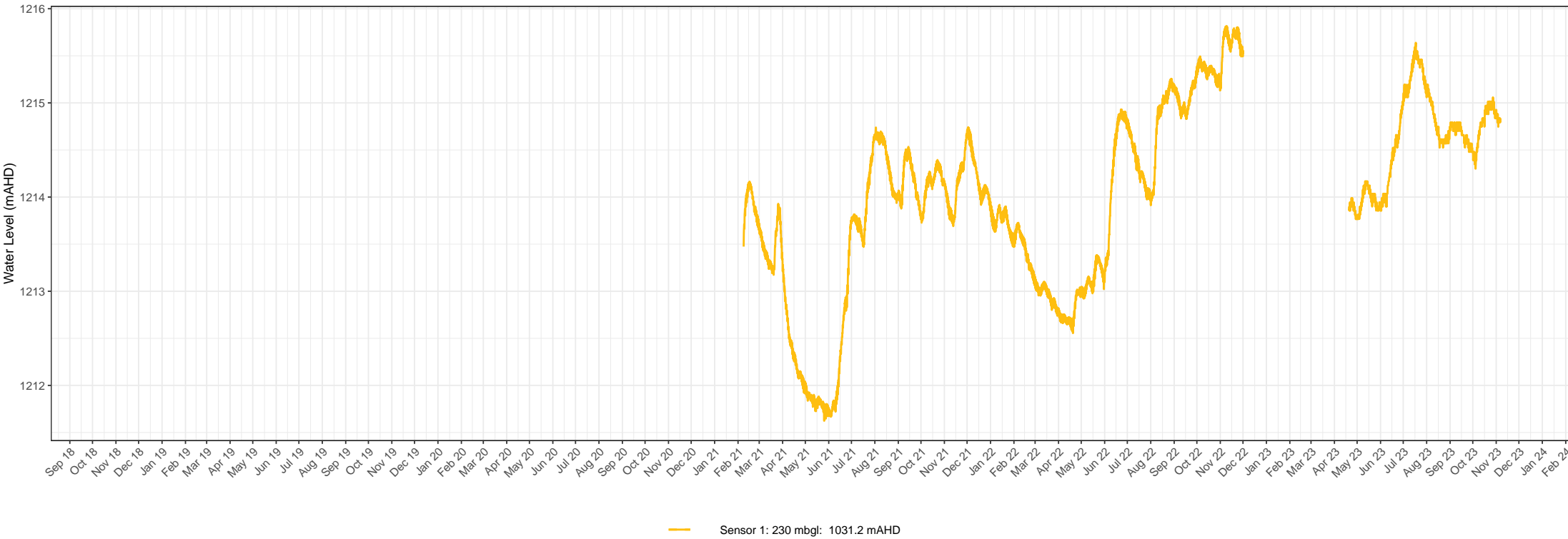
BH5202 groundwater level times series data Snowy Hydro 2.0 – Snowy Hydro Limited Groundwater monitoring and management Figure 1. 26
