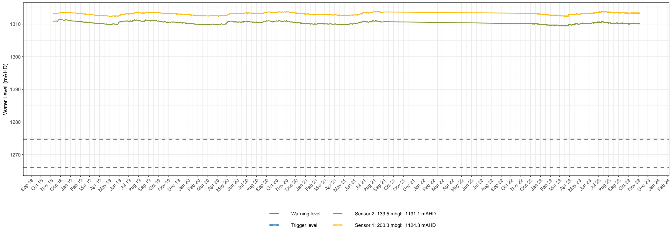
BH3107A groundwater level times series data Snowy Hydro 2.0 – Snowy Hydro Limited Groundwater monitoring and management Figure 1. 4
