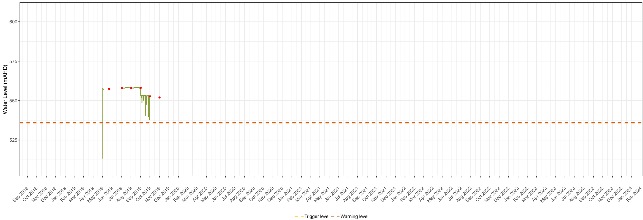
EWPB3 groundwater level times series data Snowy 2.0 – Snowy Hydro Limited Groundwater monitoring and management Figure 1. 21
