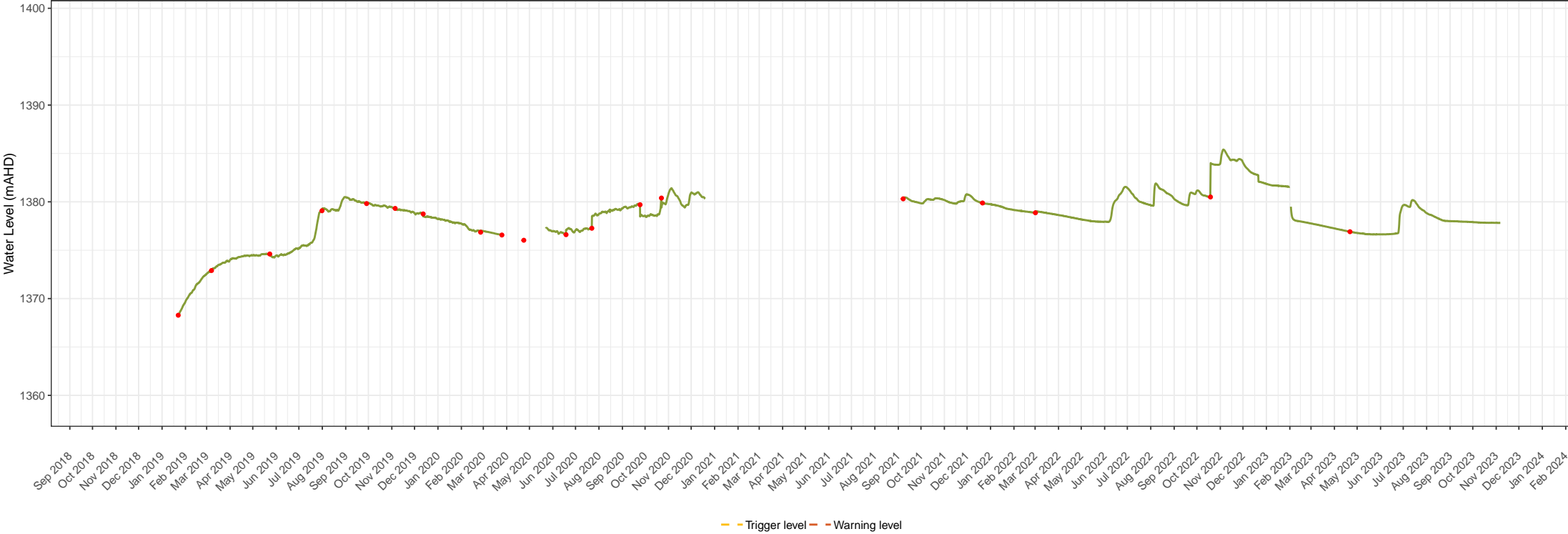
BH3102 groundwater level times series data Snowy 2.0 – Snowy Hydro Limited Groundwater monitoring and management Figure 1. 10
