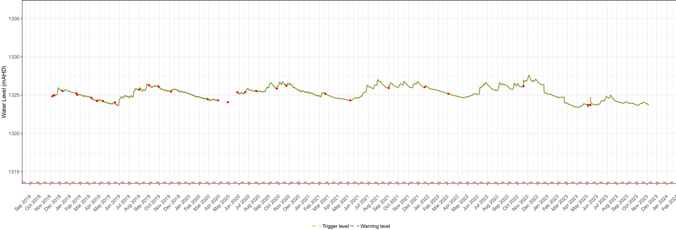
SMB05 groundwater level times series data Snowy 2.0 – Snowy Hydro Limited Groundwater monitoring and management Figure 1. 88
