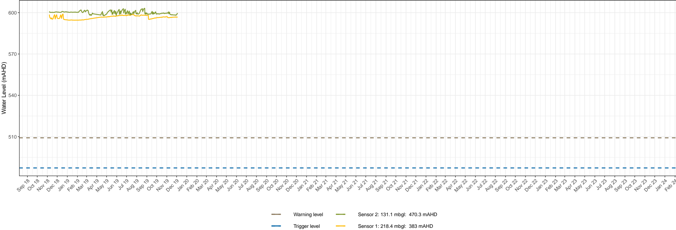
BH6103 groundwater level times series data Snowy Hydro 2.0 – Snowy Hydro Limited Groundwater monitoring and management Figure 1. 33
