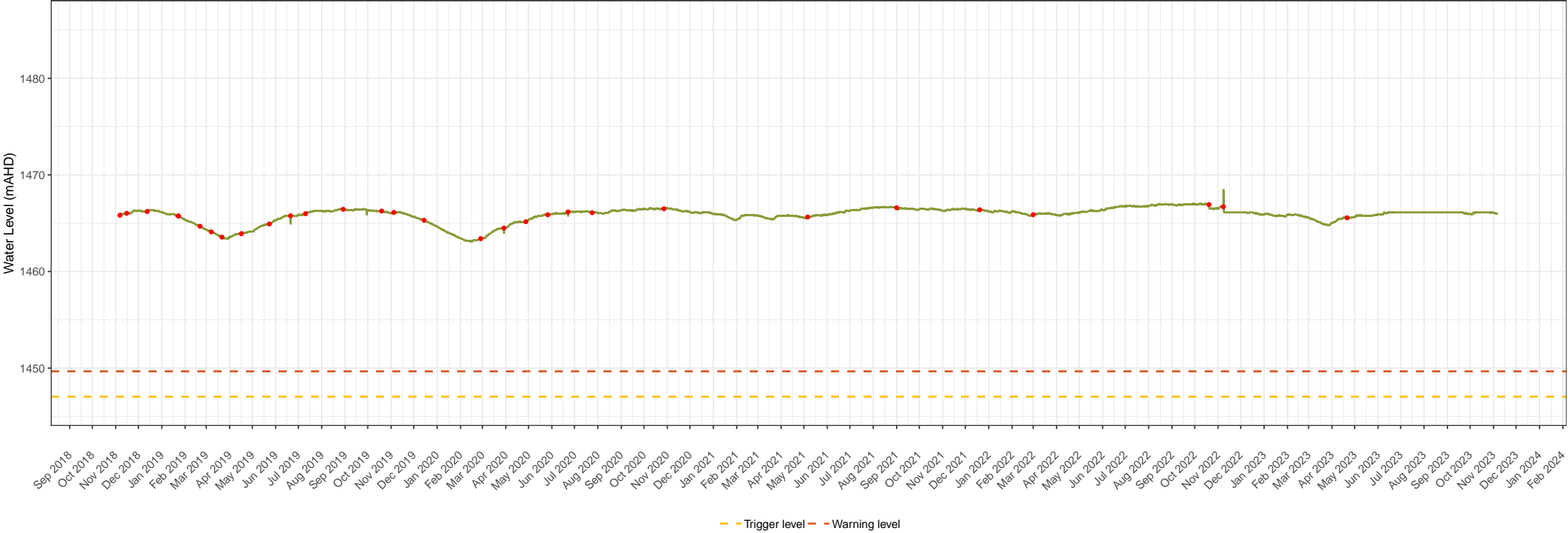
TMB03A groundwater level times series data Snowy 2.0 – Snowy Hydro Limited Groundwater monitoring and management Figure 1. 94
