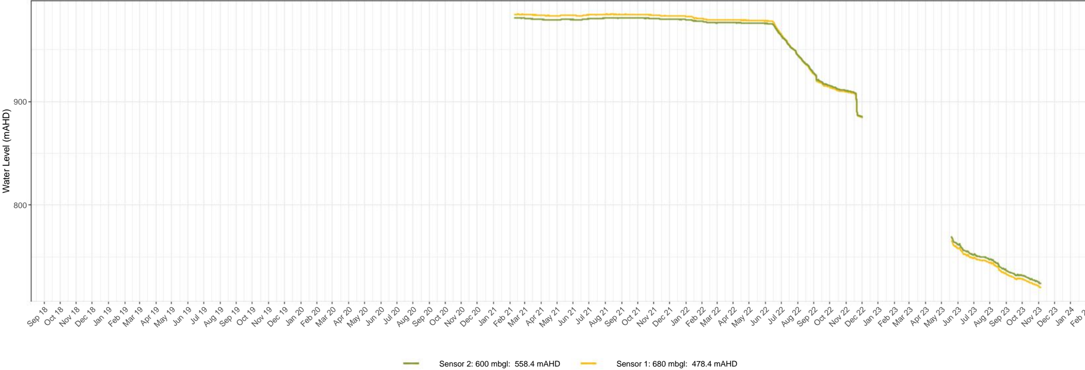
BH5206 groundwater level times series data Snowy Hydro 2.0 – Snowy Hydro Limited Groundwater monitoring and management Figure 1. 29
