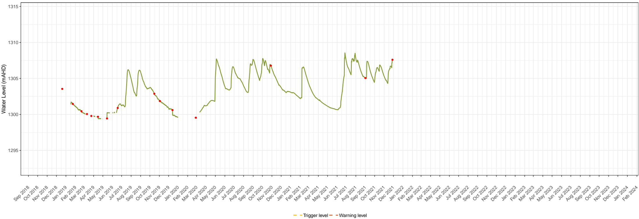
MB12A groundwater level times series data Snowy 2.0 – Snowy Hydro Limited Groundwater monitoring and management Figure 1. 38
