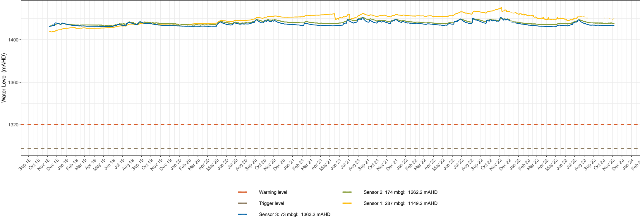
BH3104 groundwater level times series data Snowy Hydro 2.0 – Snowy Hydro Limited Groundwater monitoring and management Figure 1.2
