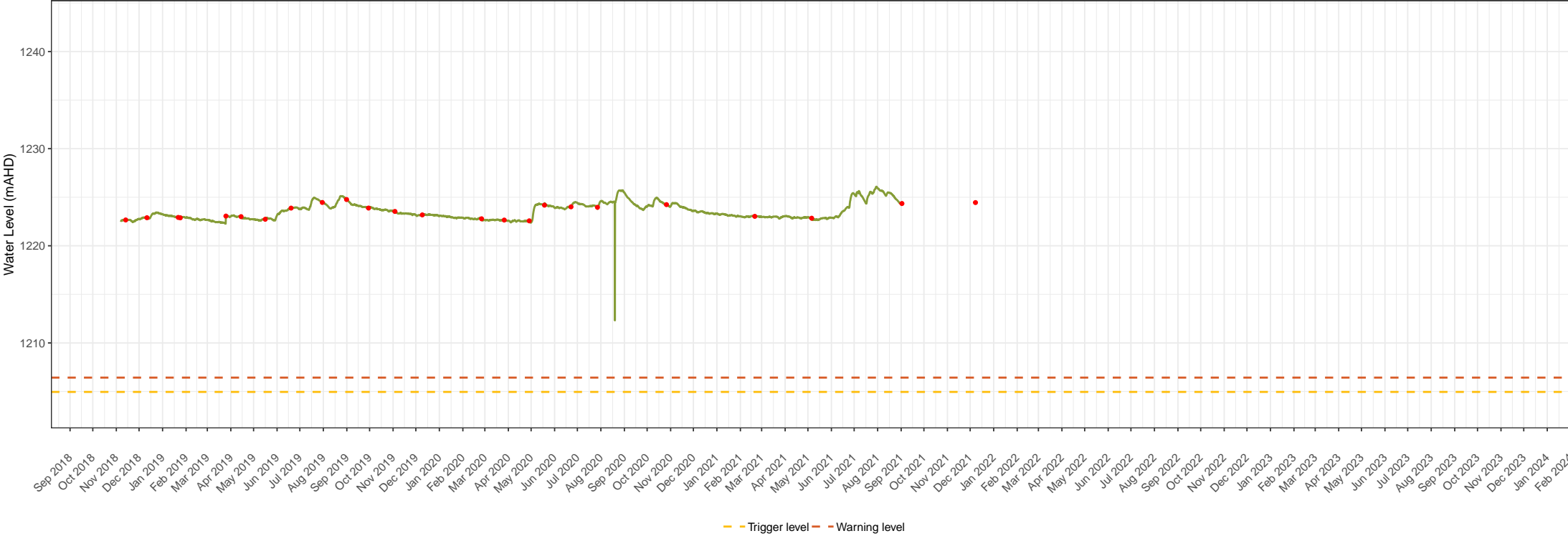
PB01 groundwater level times series data Snowy 2.0 – Snowy Hydro Limited Groundwater monitoring and management Figure 1. 45
