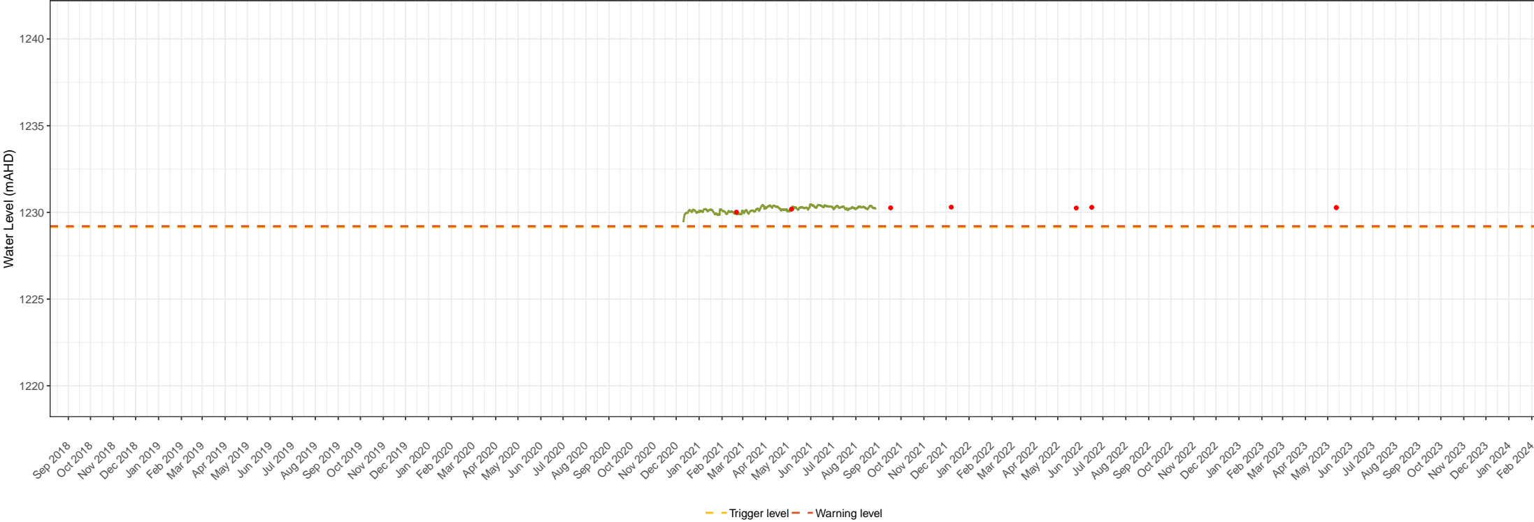
RtS_BH7A groundwater level times series data Snowy 2.0 – Snowy Hydro Limited Groundwater monitoring and management Figure 1. 78
