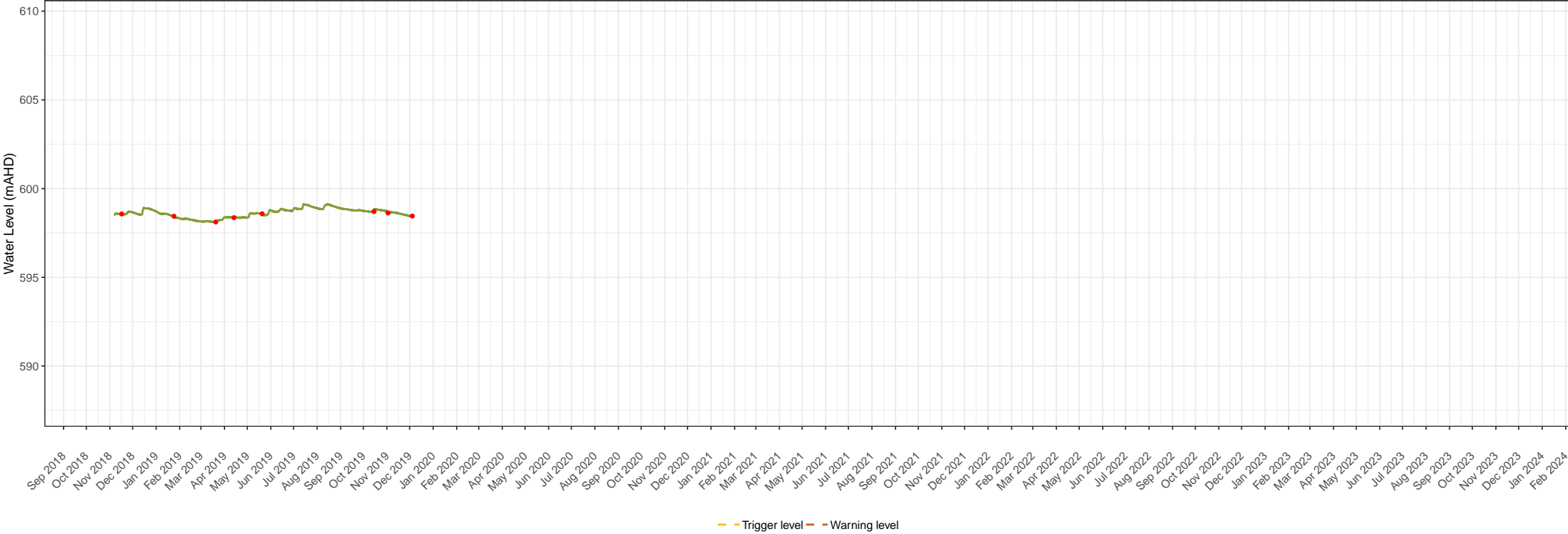
TMB05A groundwater level times series data Snowy 2.0 – Snowy Hydro Limited Groundwater monitoring and management Figure 1. 98
