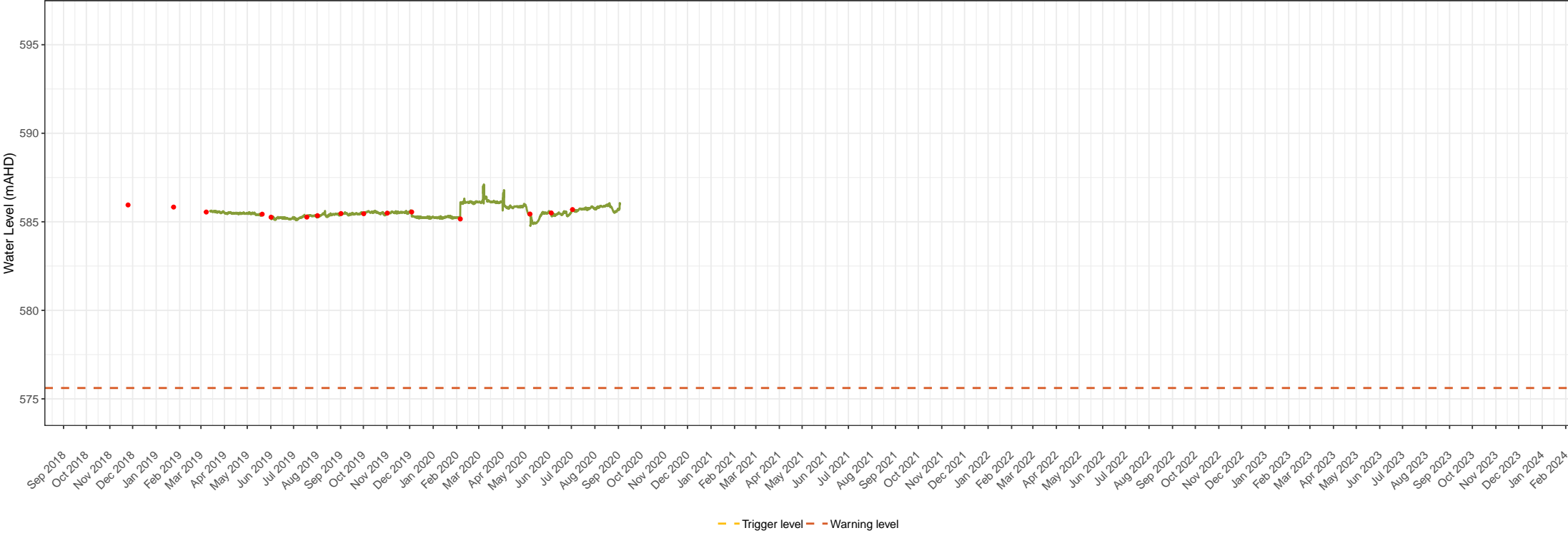
BH8101 groundwater level times series data Snowy 2.0 – Snowy Hydro Limited Groundwater monitoring and management Figure 1. 17
