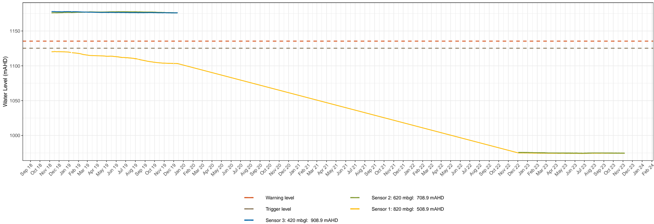
BH5102 groundwater level times series data Snowy Hydro 2.0 – Snowy Hydro Limited Groundwater monitoring and management Figure 1. 15
