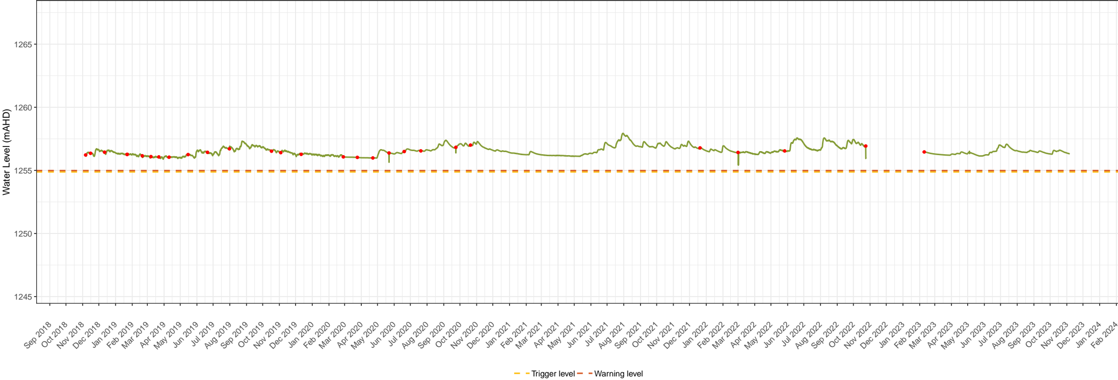
MB07A groundwater level times series data Snowy 2.0 – Snowy Hydro Limited Groundwater monitoring and management Figure 1. 33
