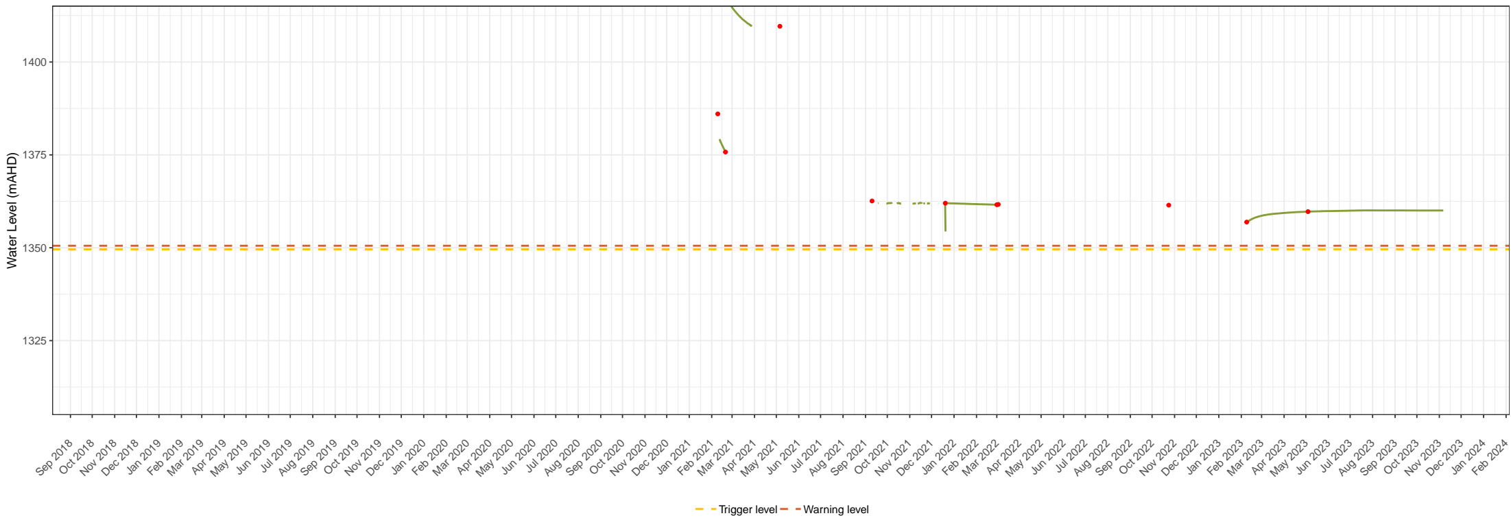
RtS_BH4B groundwater level times series data Snowy 2.0 – Snowy Hydro Limited Groundwater monitoring and management Figure 1. 75
