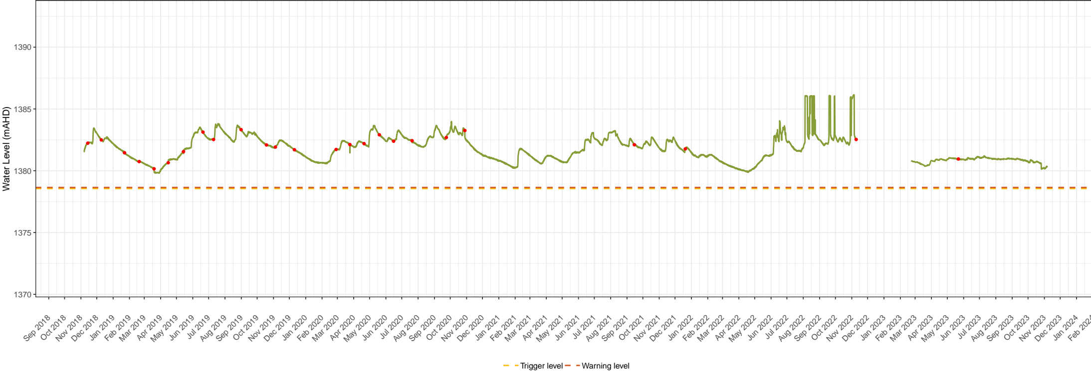
MB02 groundwater level times series data Snowy 2.0 – Snowy Hydro Limited Groundwater monitoring and management Figure 1. 27
