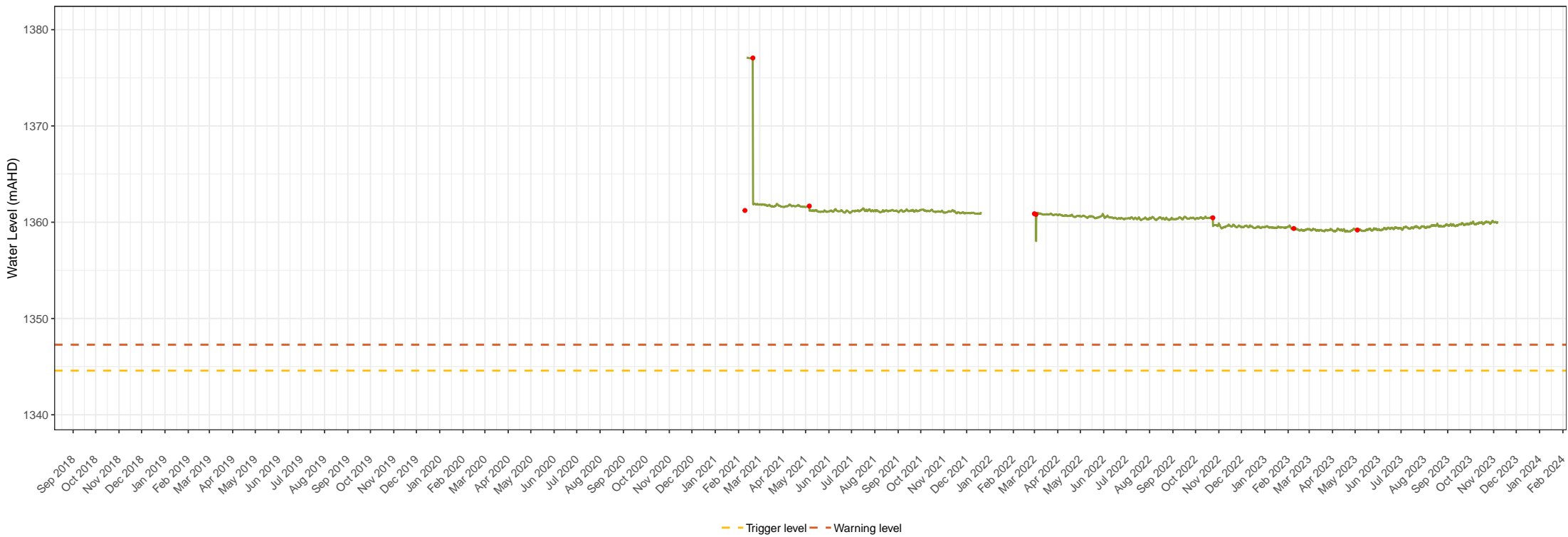
RtS_BH4A groundwater level times series data Snowy 2.0 – Snowy Hydro Limited Groundwater monitoring and management Figure 1. 74
