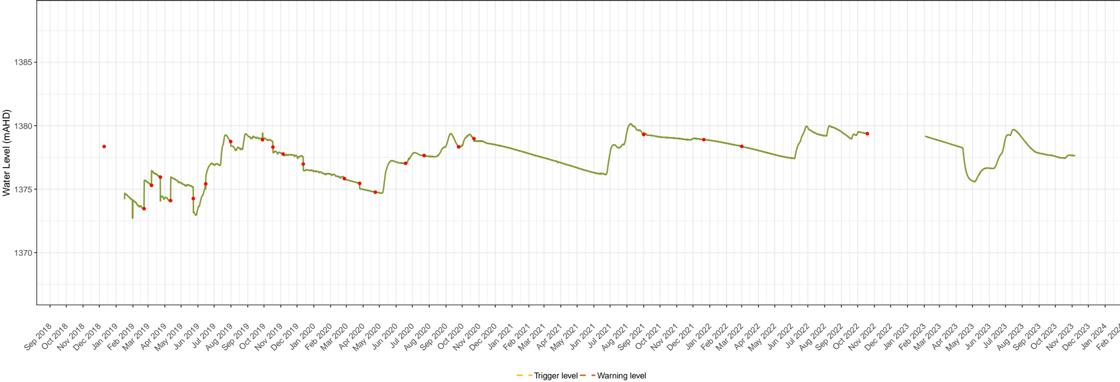
PB10 groundwater level times series data Snowy 2.0 – Snowy Hydro Limited Groundwater monitoring and management Figure 1. 50
