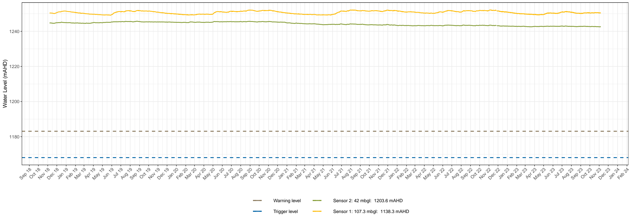
BH2102 groundwater level times series data Snowy Hydro 2.0 – Snowy Hydro Limited Groundwater monitoring and management Figure 1. 1
