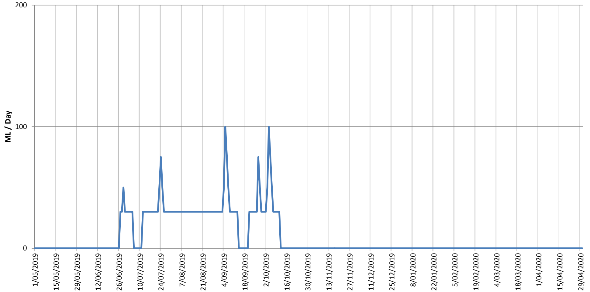
Tantangara Daily Montane Release Targets for 2019-20 Water Year
