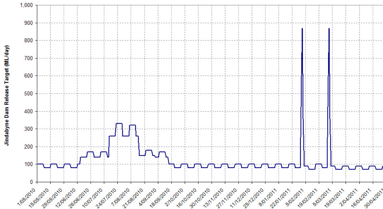
Jindabyne Daily Release Targets for 2010-11 Water Year
